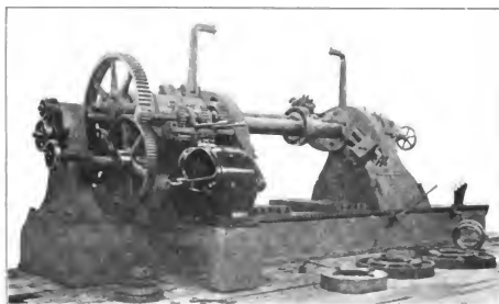
Fig. 4958. Locomotive Cylinder Boring Machine. Niles Bement-Pond Co.
